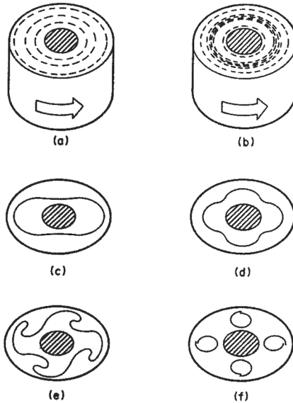
FIG. 9.3. Flow régimes in rotating-cylinder experiment: (a) uniform flow at low-temperature difference between centre and rim; (b) formation of jet flow; (c) establishment of first wave régime; (d) increased number of waves to adjust to higher temperature gradient; (e) eventual wave distortion as temperature gradient becomes too high for wave régime to account for heat transport; (f) turbulent eddies form for even more efficient energy transport at high temperature gradient. (After R. Hide.)
